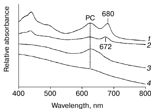
Fig. 1. Absorption spectra of chlN − cells grown in iron-sufficient (1, 3) and -deficient (2, 4) media. The spectrum of the chlN − mutant was determined after growth in continuous light (1, 2) or under LAHG conditions (3, 4) for two weeks.
